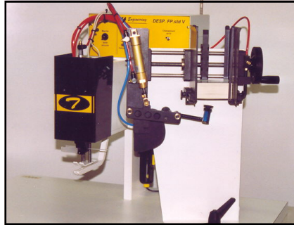
Model with 1 automatic tag dispenser
