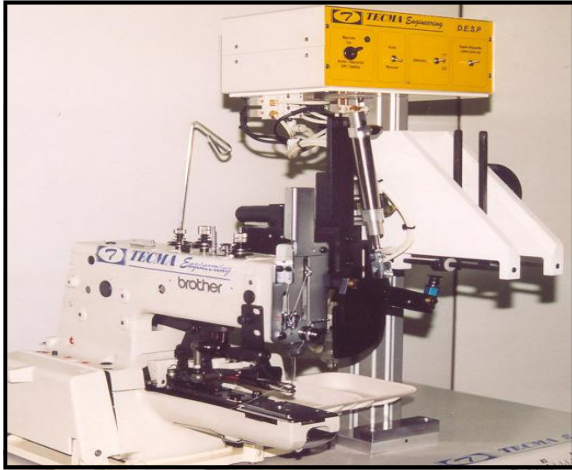
MODEL DESP with 1 automatic tag dispenser.
