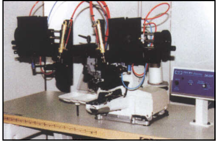
MODEL DE2SP with 2 automatic tag dispensers.
