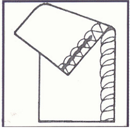
3 hilos 1 aguja
